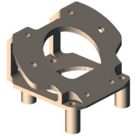
Star Tracker Interface Bracket (Titanium)
